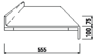
VT3 – Vanity Top for Inset Hand Wash Basin, with Upstand
