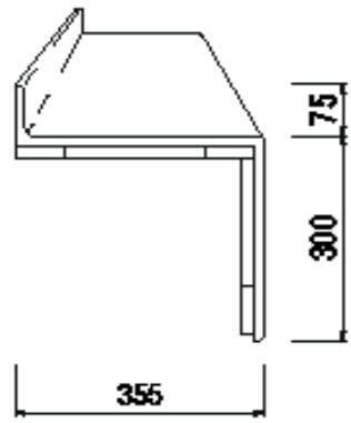
VT1 – Vanity Top for Semi-recessed Hand Wash Basin, with Upstand
