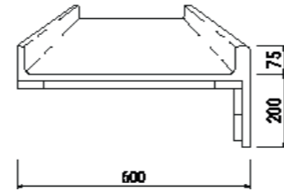
BC1 – Baby Change Top with Front and Rear Upstands
